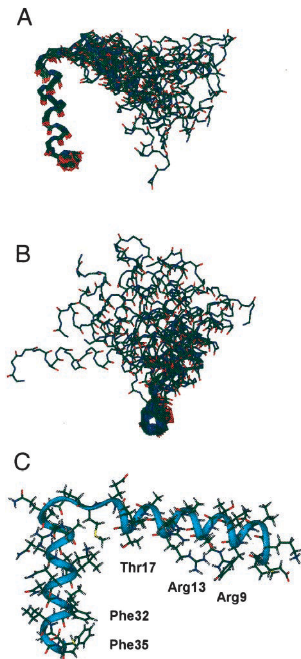
FIGURE 4 Structures of PLB[1–36] deduced from NMR data. (A and B) Orthogonal view of 18 structures with no violations >0.2 Å, superimposed on the C\alpha of the residues in the carboxyl-terminal helix. The amino-terminal helix is dispersed in a cone with an opening of approximately 80^\circ . The interhelix angle is 80 \pm 20^\circ ( n = 18 ). (C) The structure with least NOE violations (three violations >0.1 Å, no violations >0.2 Å). Some of the side chains are marked.
