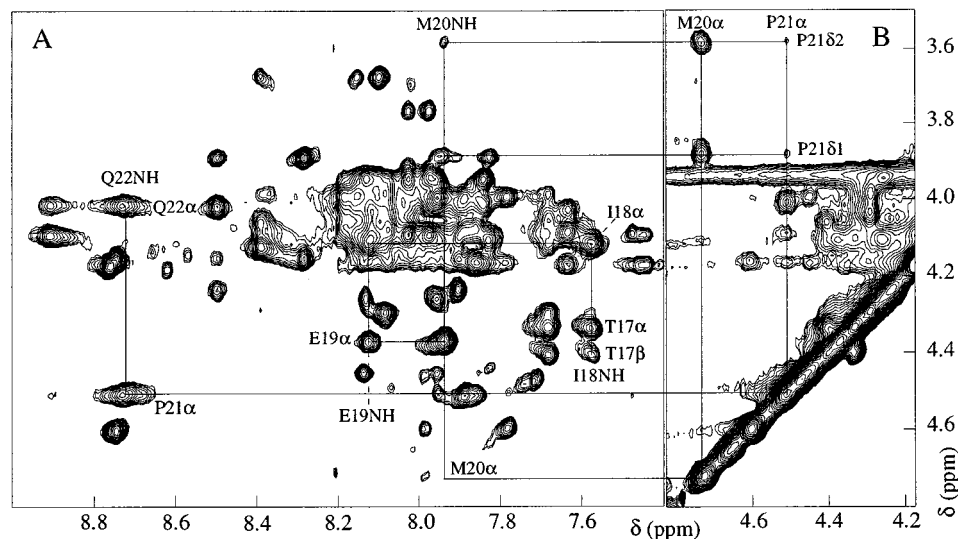
FIGURE 2 Expansions from NOESY spectra acquired at 17°C at 160-ms mixing times on 3 mM PLB[1–36] in 63% H 2 O/7% D 2 O/30% d 3 -TFE, pH 3.05, in the presence of 6 mM d 10 -DTT. (A) Fingerprint region. The cross-peaks generated by the correlations NH i C \alpha H i are marked. (B) Region showing cross-peaks from the turn Glu19, Met20, Pro21.
